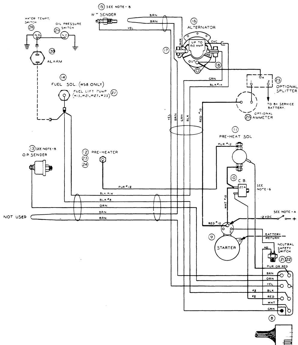
WIRING DIAGRAM
