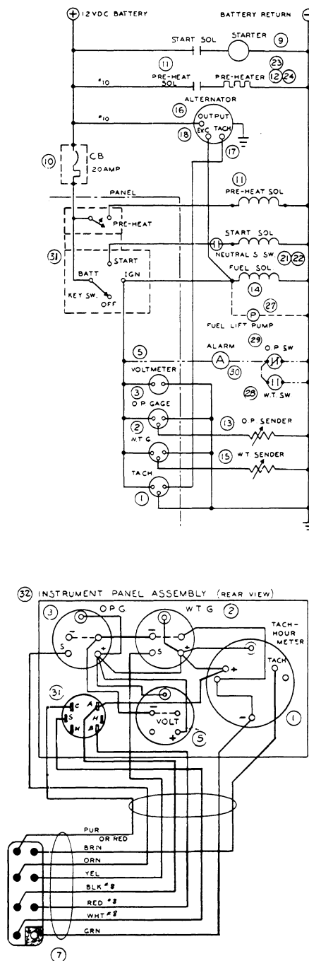
SCHEMATIC DIAGRAM
