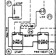
REMOTE CONTROL PANEL (REAR VIEW)
