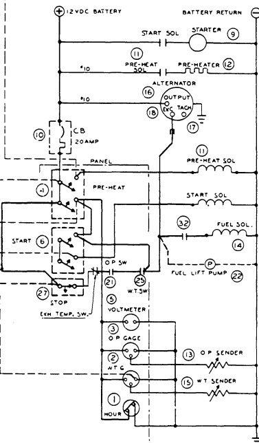
SCHEMATIC DIAGRAM
