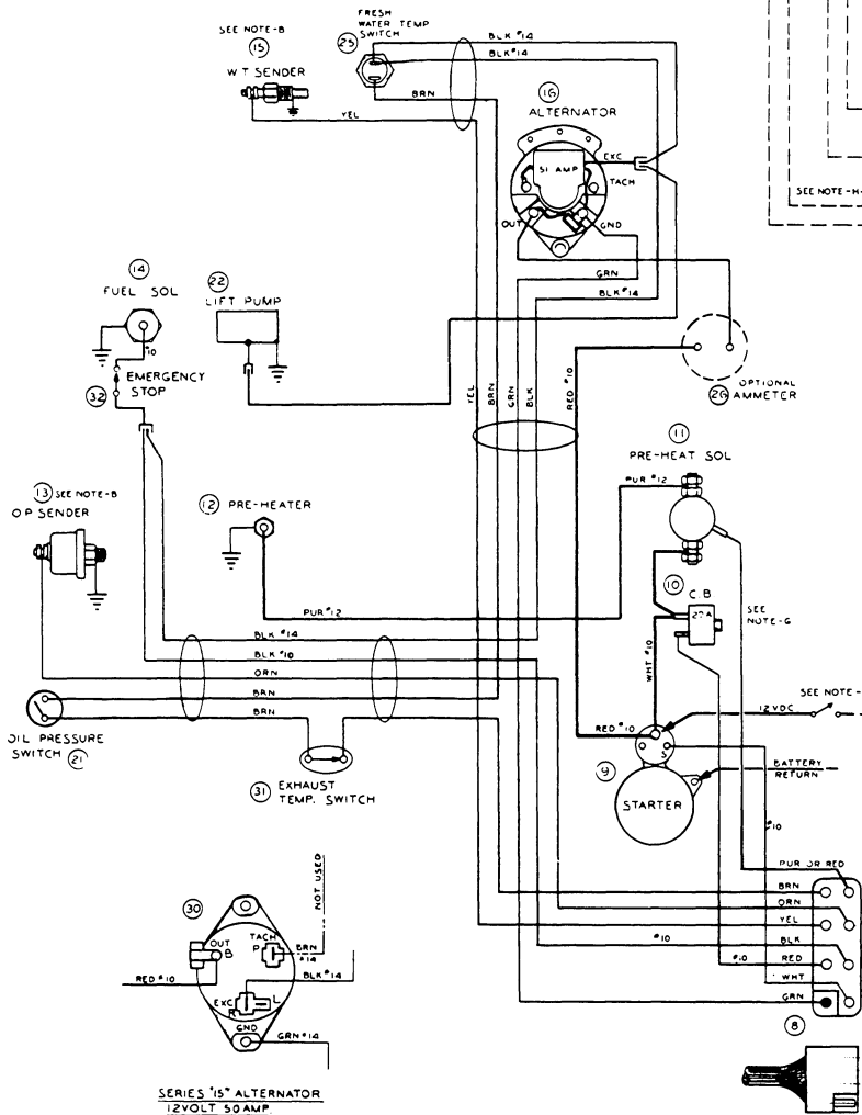
WIRING DIAGRAM
