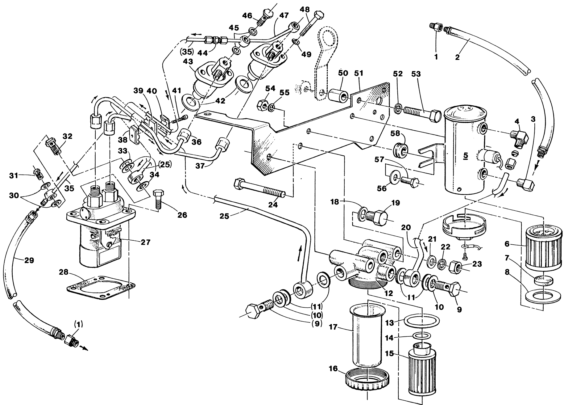
WESTERBEKE 15 - FUEL SYSTEM
