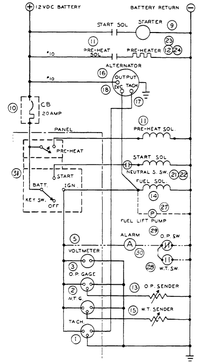
SCHEMATIC DIAGRAM.
