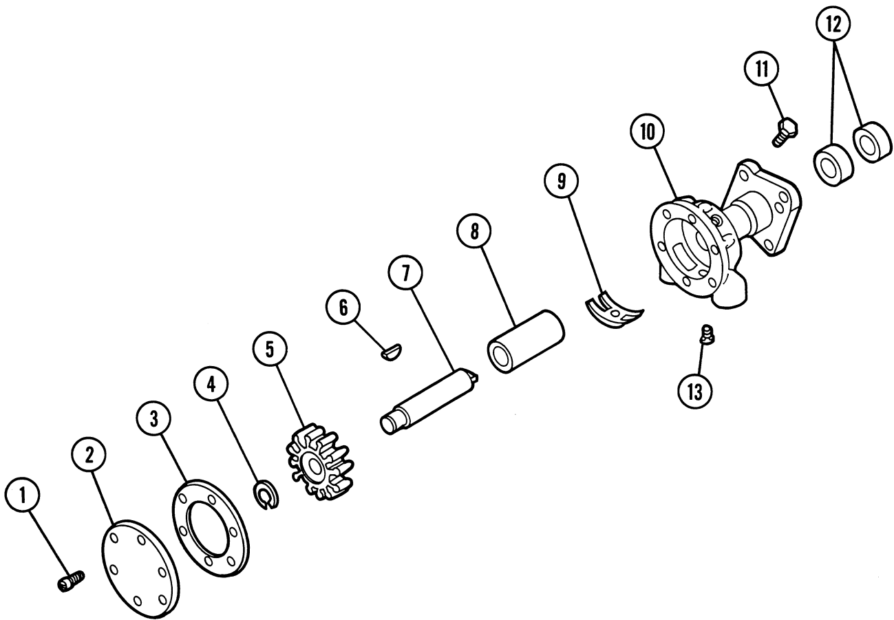
300986 Pump Assembly
