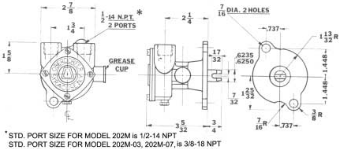
202M, 202M-03, 202M-07 DIMENSIONS
