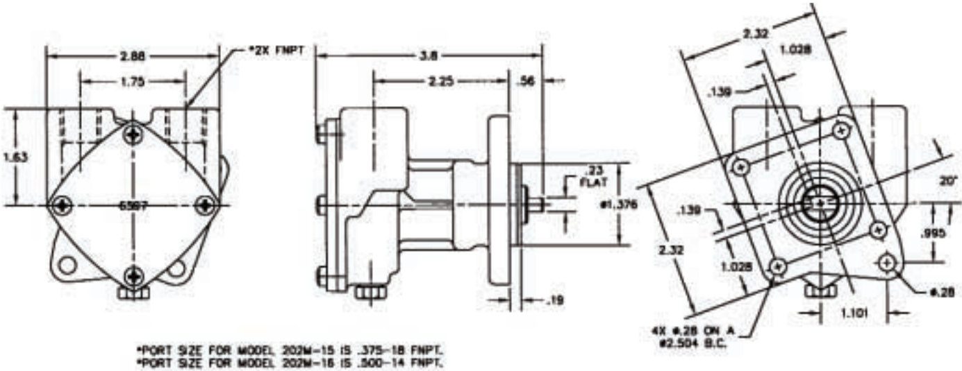
202M-15, 202M-16 DIMENSIONS
