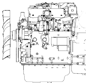
4LE2X: 31.60 in. (803 mm)
