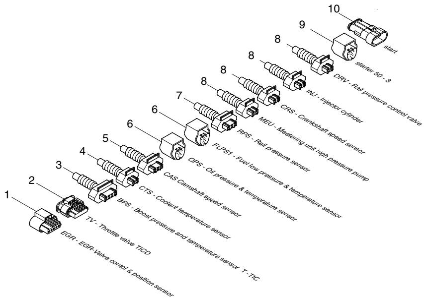
engine wiring harness C81
