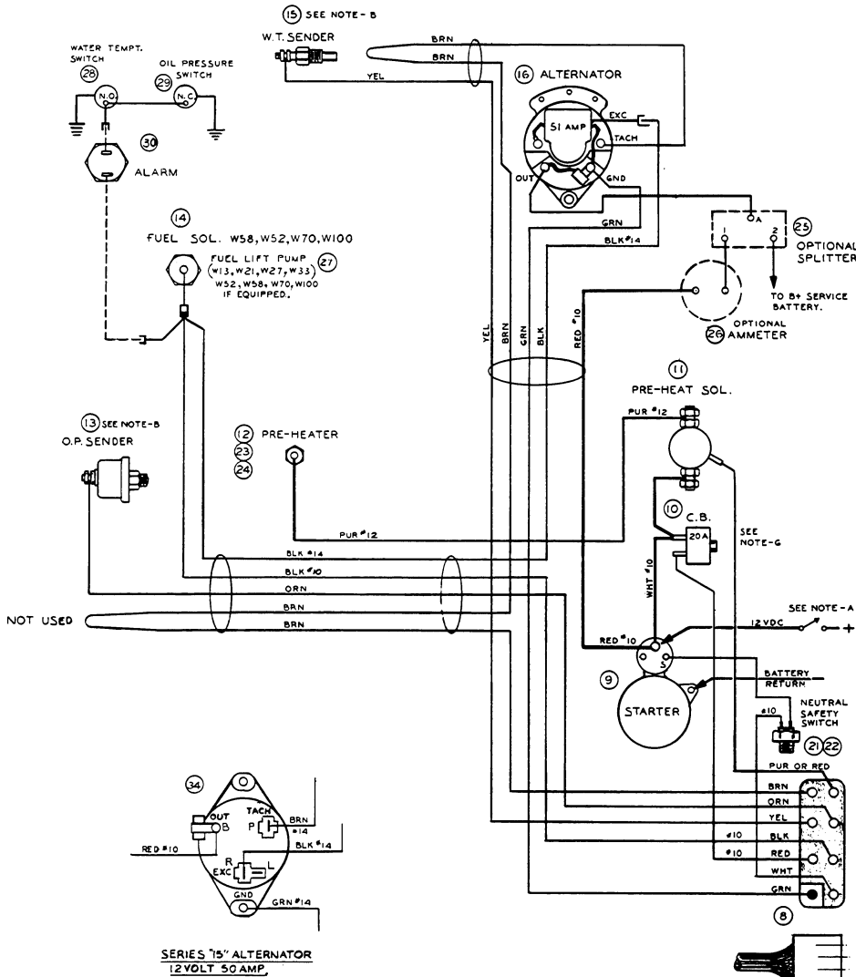
WIRING DIAGRAM. 33685
