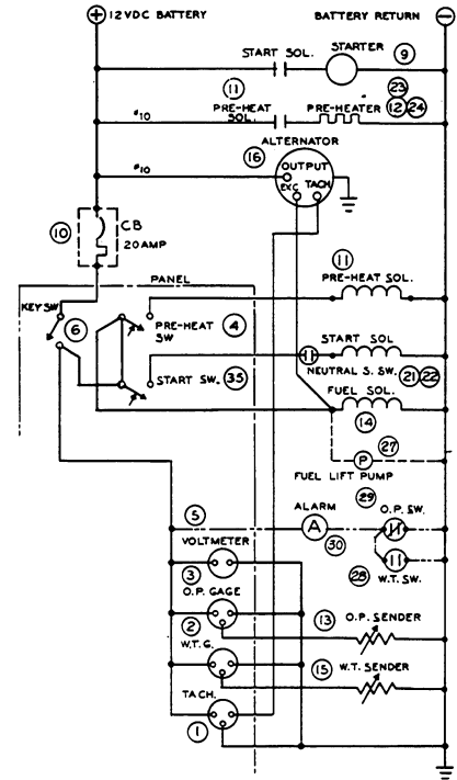
SCHEMATIC DIAGRAM.
