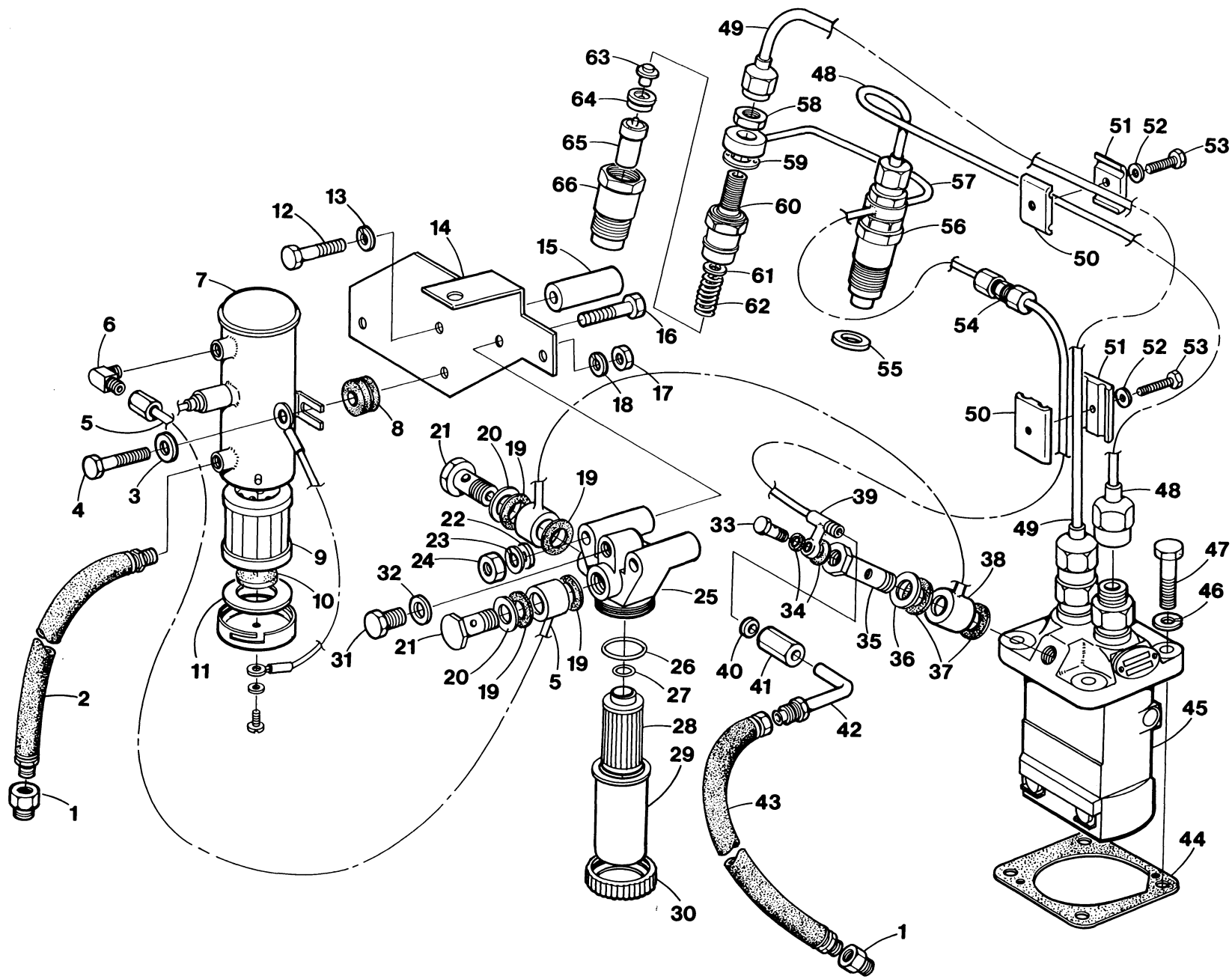
WESTERBEKE 10TWO - FUEL SYSTEM
