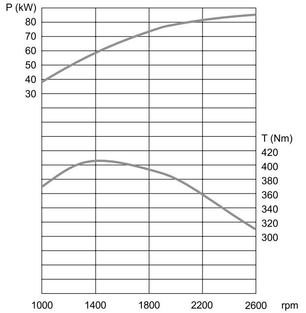
Engine TCD 2010 L4
