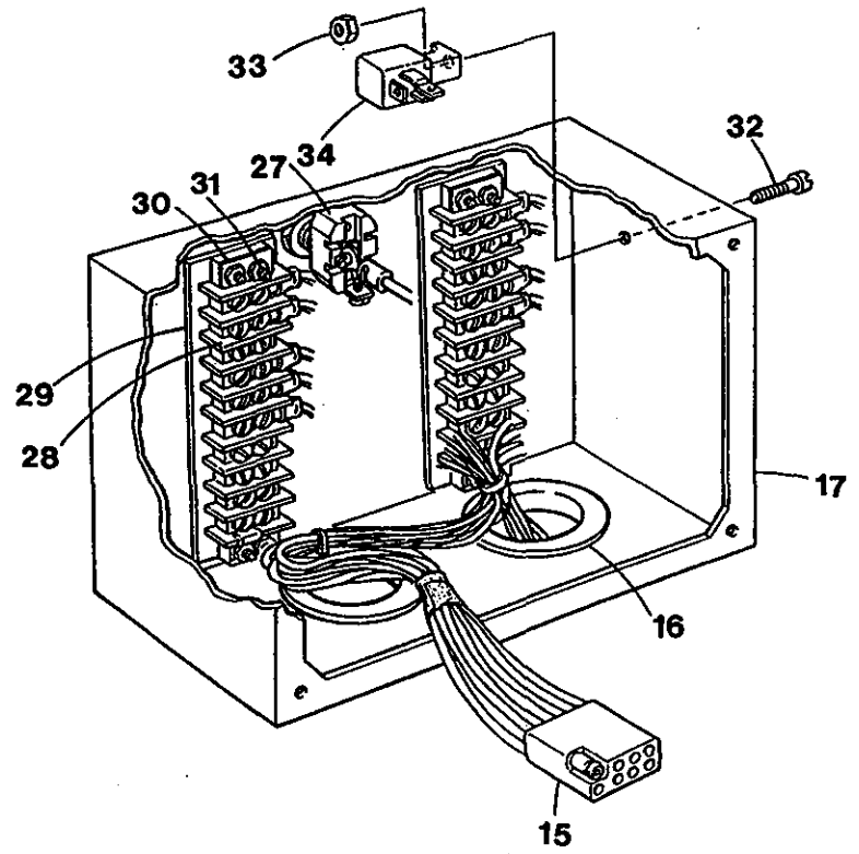
WESTERBEKE 5.0 BCD GENERATOR - CONTROL PANEL
