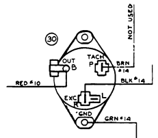
SERIES '15' ALTERNATOR 12VOLT 30AMP.
