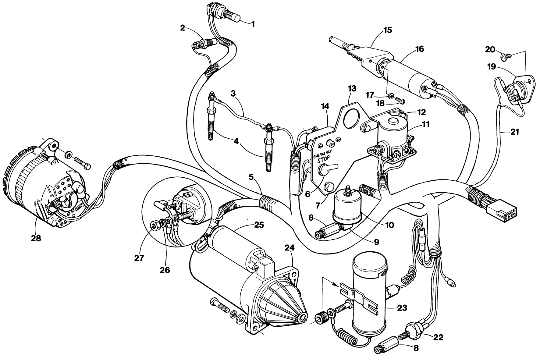
WESTERBEKE 3KW - GENERATOR HARNESS
