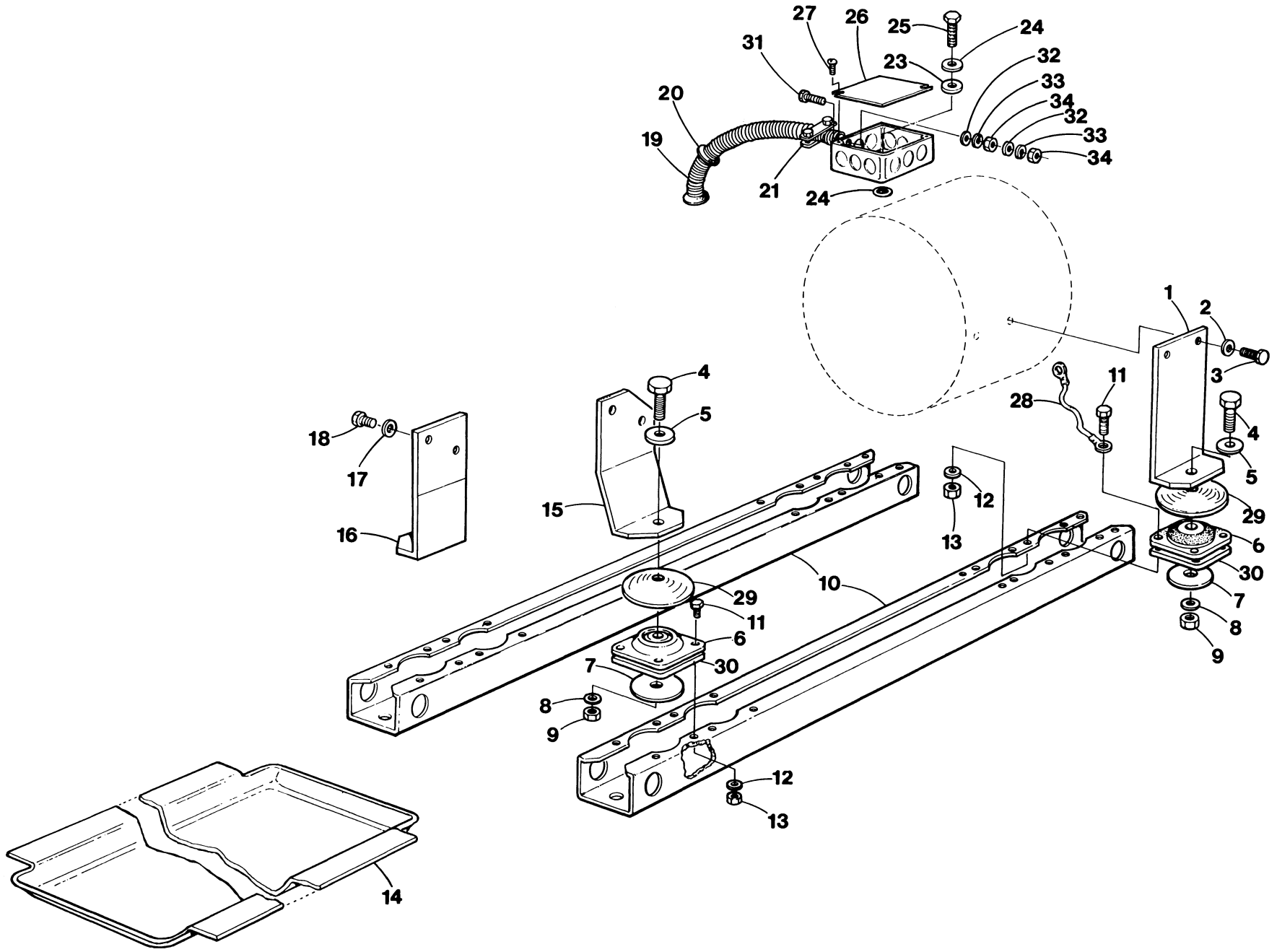
WESTERBEKE 3KW - GENERATOR MOUNTING SYSTEM
