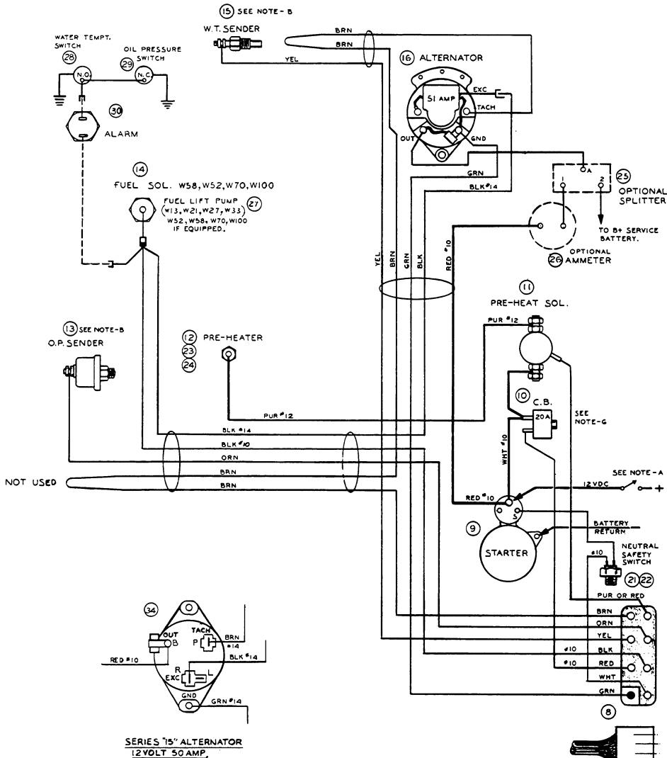
WIRING DIAGRAM. 33685
