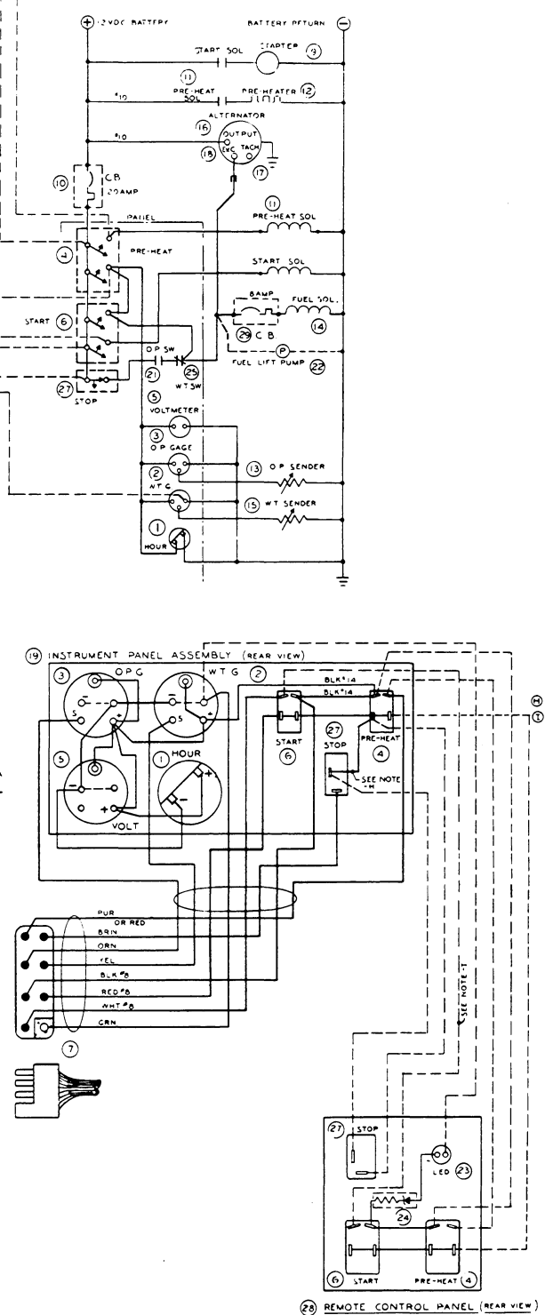
SCHEMATIC DIAGRAM
