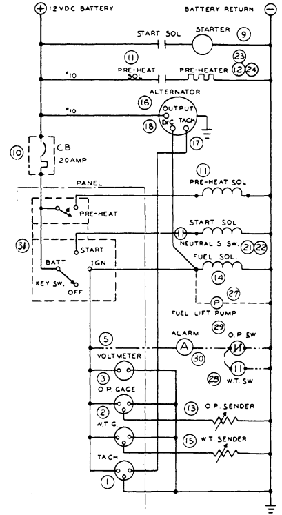
SCHMATIC DIAGRAM
