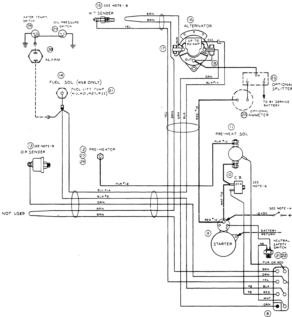
WIRING DIAGRAM
