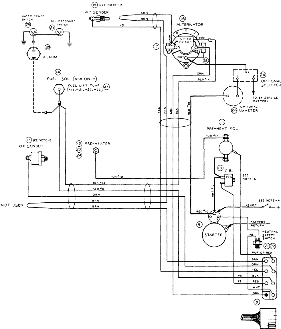
WIRING DIAGRAM
